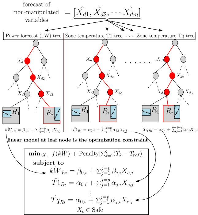
Fig. 6. DR synthesis with thermal comfort constraints. Each tree is responsible for contributing one constraint to the demand response optimization.
