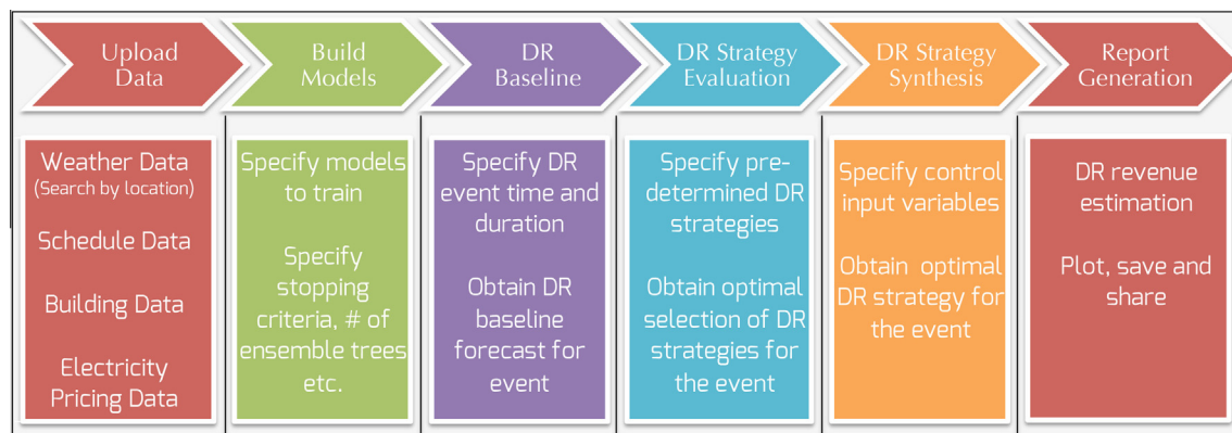
Fig. 9. DR-Advisor workflow.
