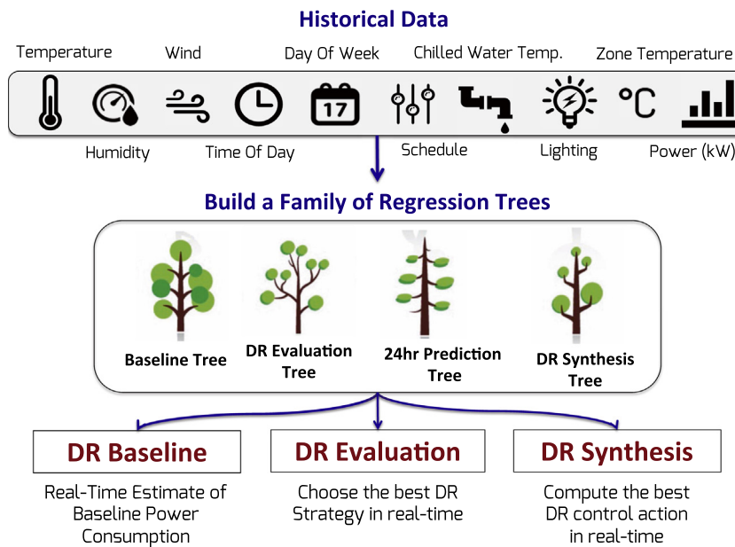
Fig. 2. DR-Advisor architecture.
