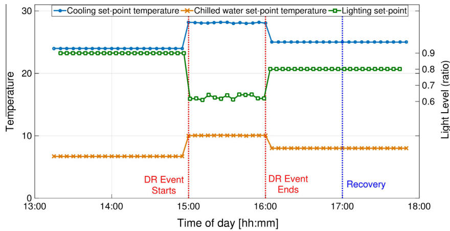
Fig. 16. Optimal DR strategy as determined by the mbCART algorithm.
