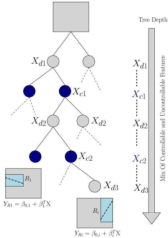
Fig. 4. Example of a regression tree with linear regression model in leaves. Not suitable for control due to the mixed order of the controllable X_c (solid blue) and uncontrollable X_d features. (For interpretation of the references to color in this figure legend, the reader is referred to the web version of this article.)
