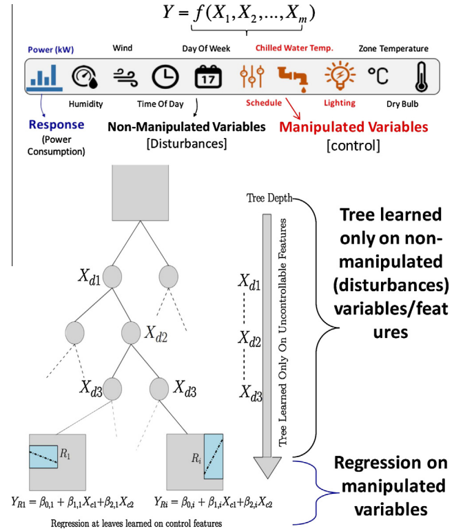
Fig. 5. Example of a tree structure obtained using the mbCRT algorithm. The separation of variables allows using the linear model in the leaf to use only control variables.
