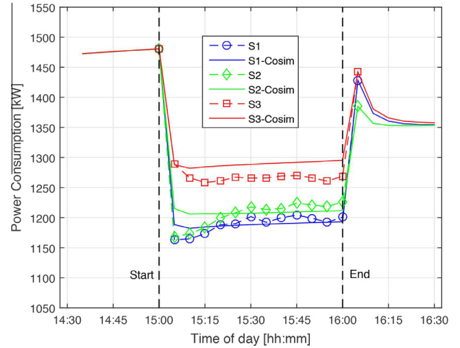
Fig. 14. Prediction of power consumption for 3 strategies. DR Evaluation shows that Strategy 1 (S1) leads to maximum power curtailment.
