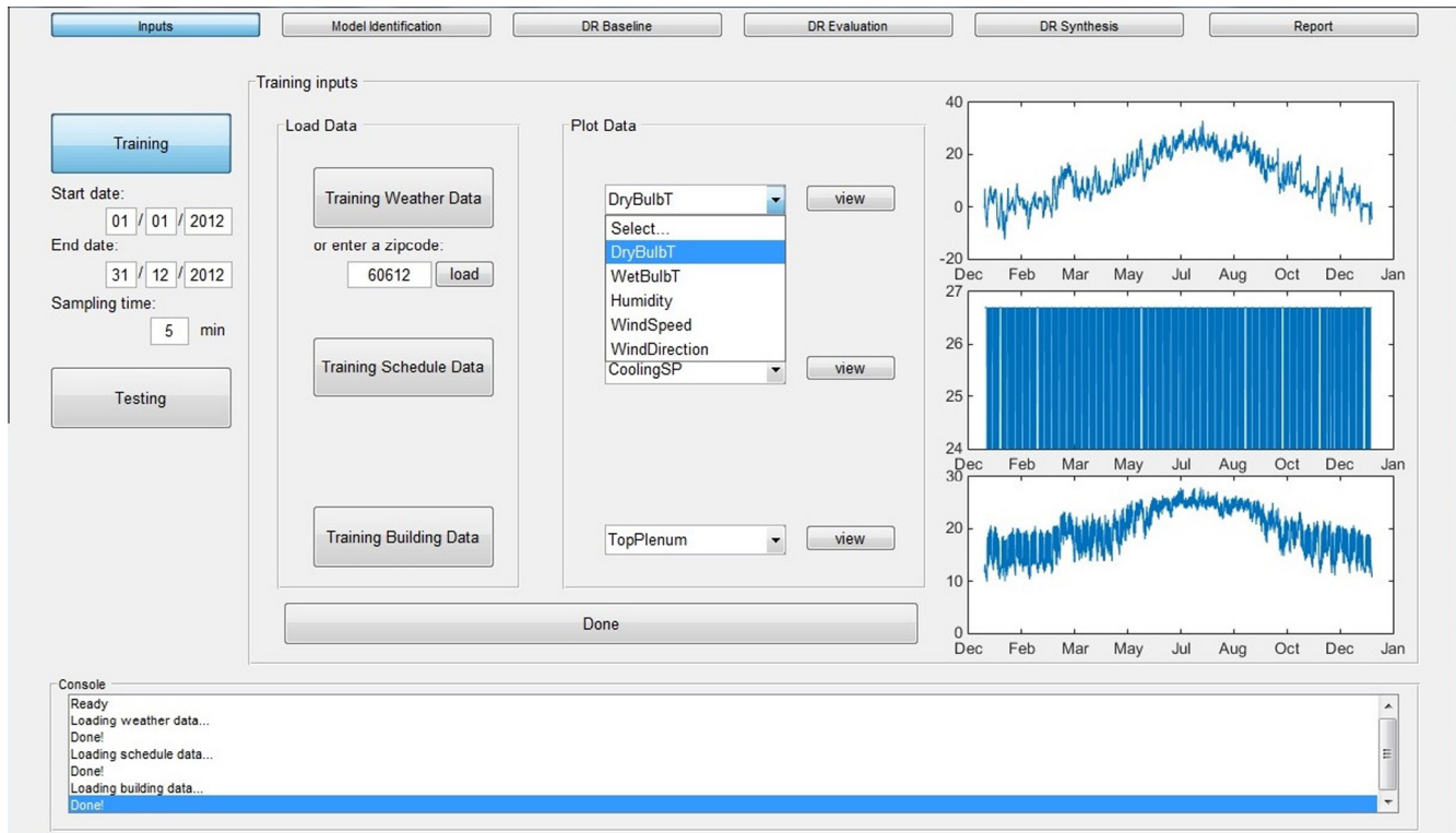
Fig. 8. Screenshot of the DR-Advisor MATLAB based GUI.
