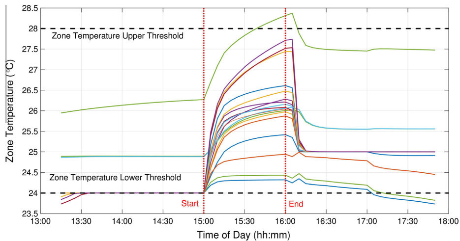
Fig. 17. The mbCART algorithm maintains the zone temperatures within the specified comfort bounds during the DR event.
