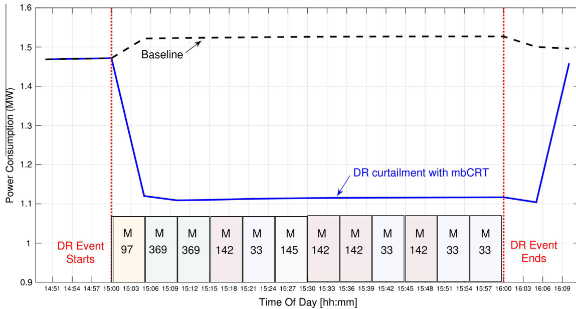
Fig. 18. Zoomed in view of the DR synthesis showing how the mbCRT algorithm selects the appropriate linear model for each time-step based on the forecast of the disturbances.
