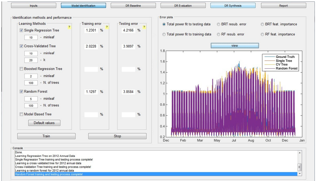
Fig. 10. DRAdvisor model identification tab.
