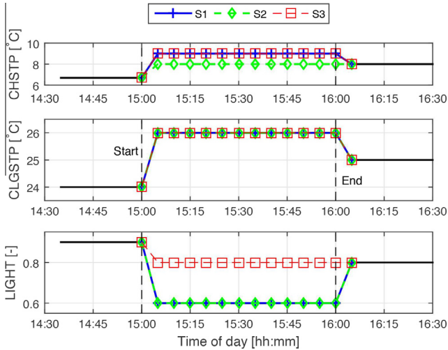
Fig. 13. Rule-based strategies used in DR evaluation. CHSTP denotes Chiller set point and CLGSTP denotes Zone Cooling temperature set point.
