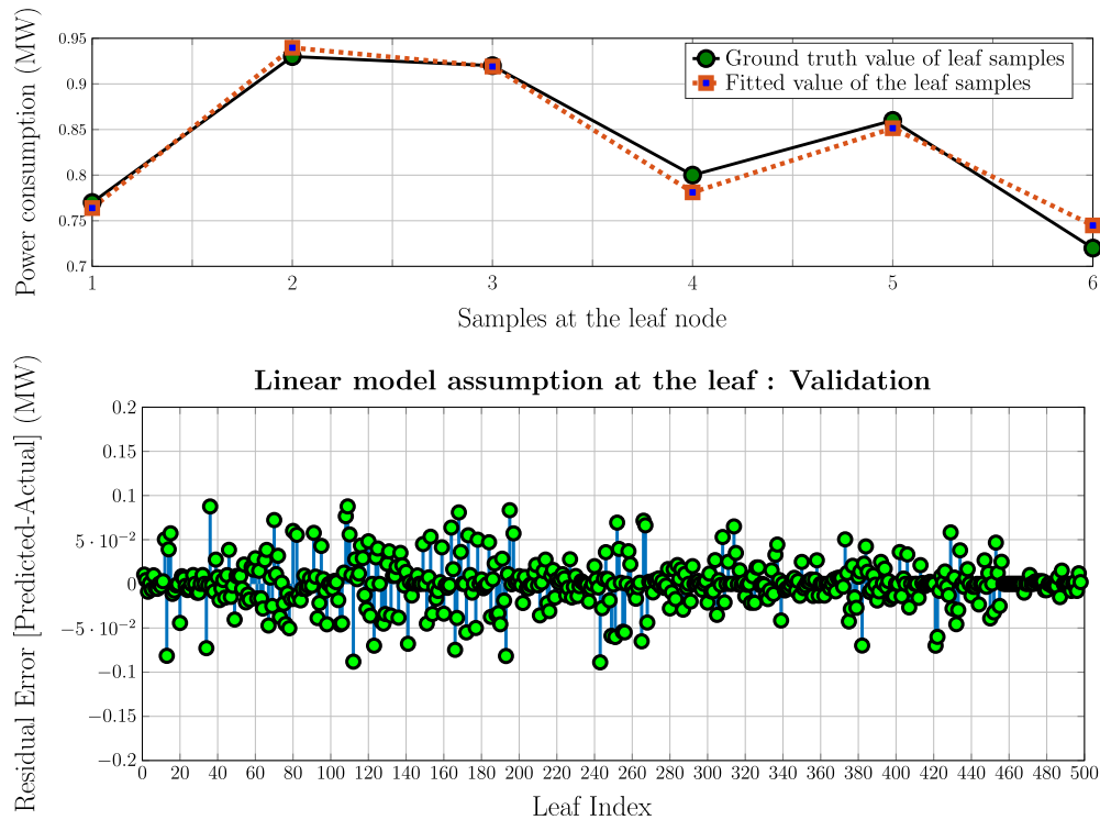
Fig. 7. Linear model assumption at the leaves. The top figure shows the comparison between fitted values and ground truth values of power consumption for one of the leaves in the power consumption prediction tree. The bottom figure shows the residual error between fitted and actual power consumption values for all the leaf nodes of the tree.
