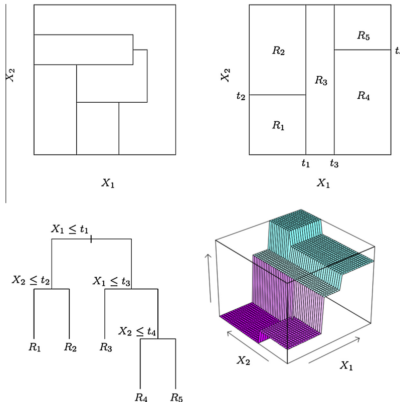
Fig. A.19. Top right: 2D feature space by recursive binary splitting. Top left: partition that cannot be obtained from recursive binary splitting. Bottom left: tree corresponding to the partition. Bottom right: perspective plot of the prediction surface.
