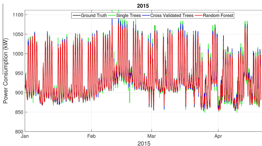
Fig. 12. Model validation for the clinical research building at Penn.
