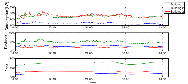
Figure 2: Power-vol. deviation-price for 3 buildings
