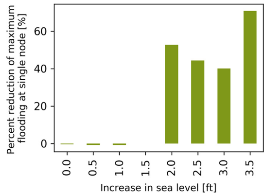
Fig. 8. Percent reduction of maximum flooding at an individual node with MPC compared to tide gate scenario given increasing sea level.
