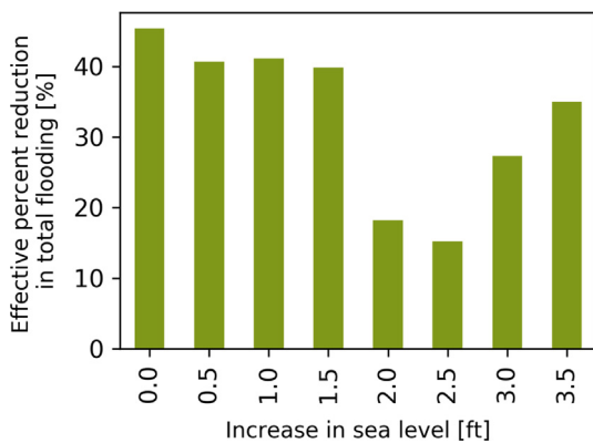
Fig. 7. Effective percent total flood reduction in MPC compared to tide gate scenario given increasing sea level.
