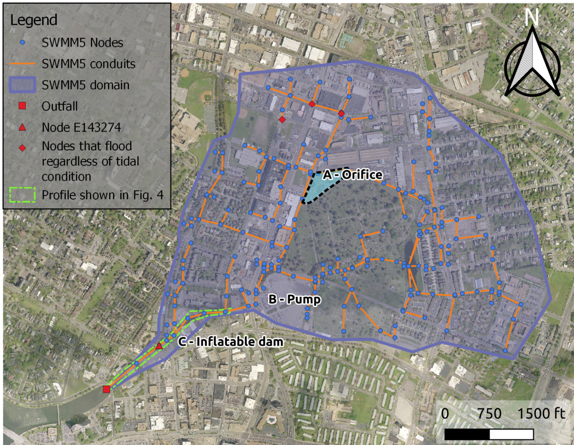
Fig. 3. SWMM5 model of the study area and simulated actuators.
