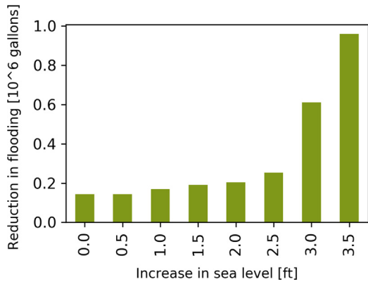
Fig. 6. Flood reduction in MPC compared to tide gate scenario given increasing sea level.
