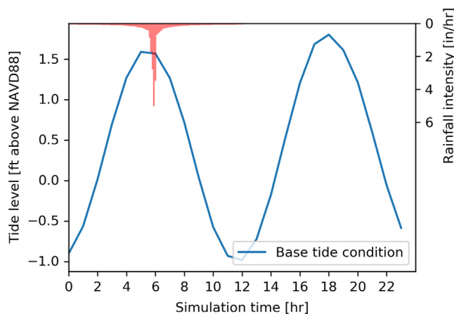
Fig. 2. Design storm and base tide condition.
