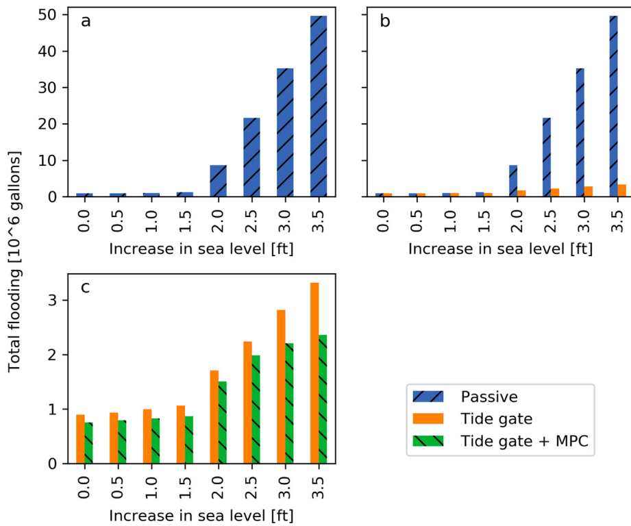
Fig. 5. Flooding with sea level increases in (a) passive scenario, (b) passive compared to tide gate scenario, and (c) tide gate compared to MPC with tide gate scenario.
