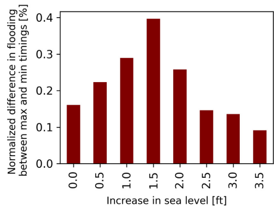
Fig. 11. Difference between the flood volume caused by the worst-case scenario timing and the best-case scenario timing normalized by the average flood volume for each sea level increase.
