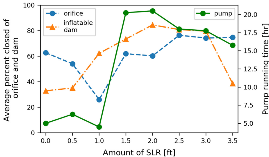
Fig. 9. Use of controls in each of the SLR scenarios - the average percent closed of the orifice and inflatable dam and running time of the pump for SLR from 0 to 3.5 ft.
