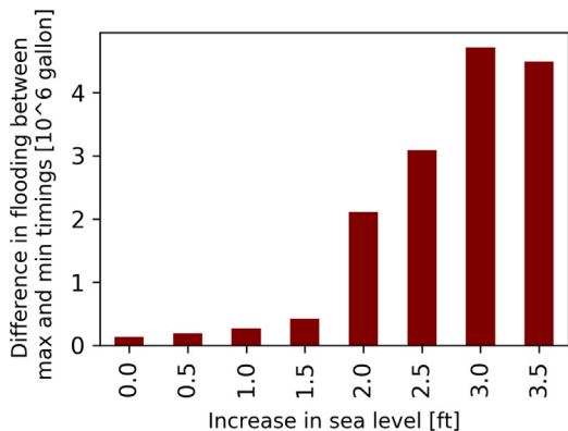
Fig. 10. Difference between the flood volume caused by the worst-case scenario timing and the best-case scenario timing.
